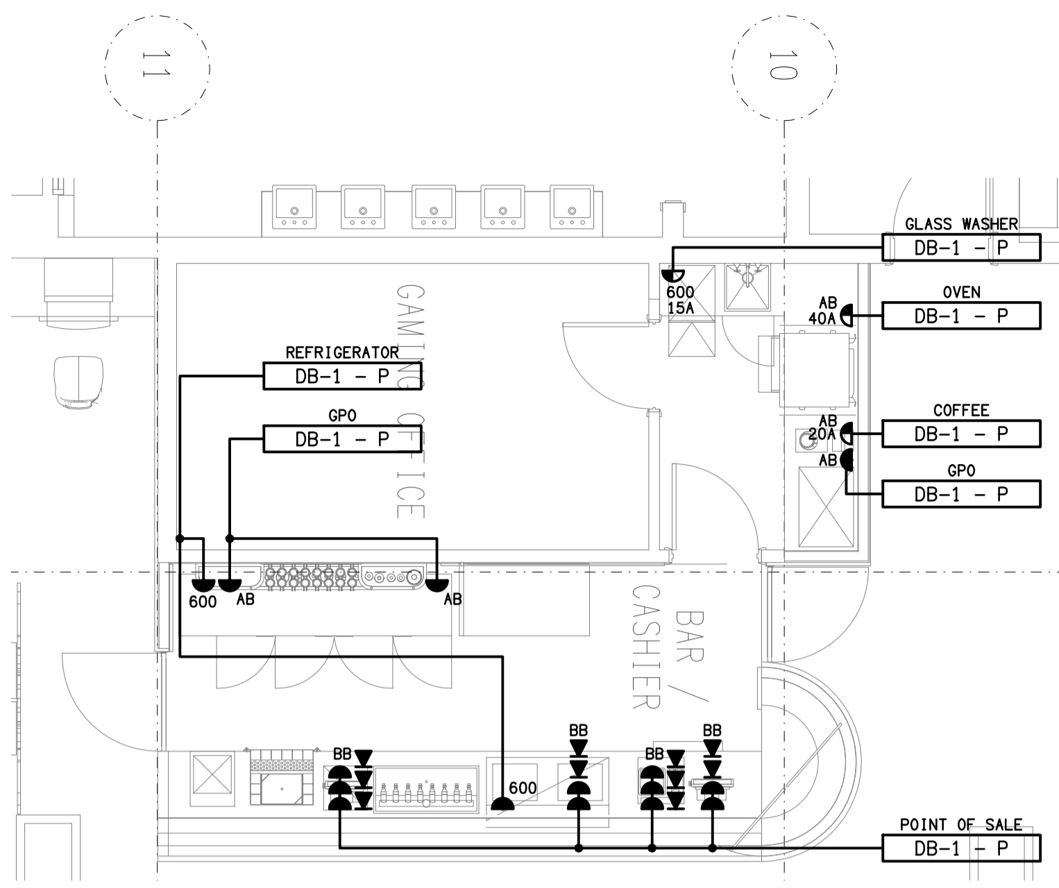
DETAIL A BAR / CASHIER FLOOR PLAN SCALE 1:50
